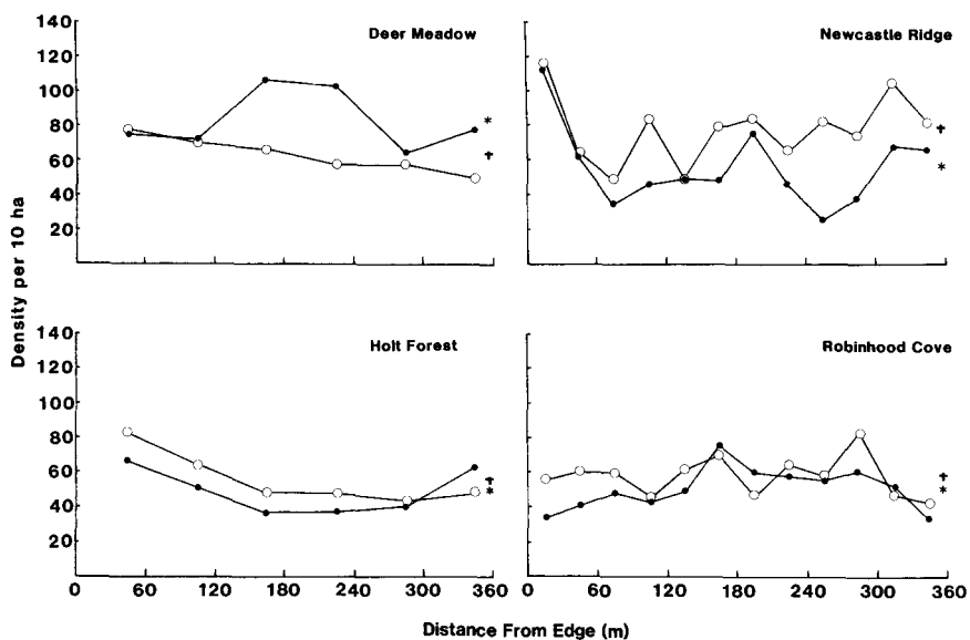
FIG. 2. Density of passerines per 10 ha at different distances from the edge. Closed circles denote 1984 results, open circles, 1985 results. Points are located at segment midpoints. Asterisks are 1984 mean densities, crosses are for 1985 means.
