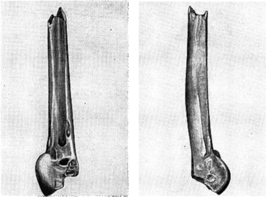
FIG. 1. Tibiotarsus of Boreortalis laesslei . Anterior (left) and external views. About two times natural size.
