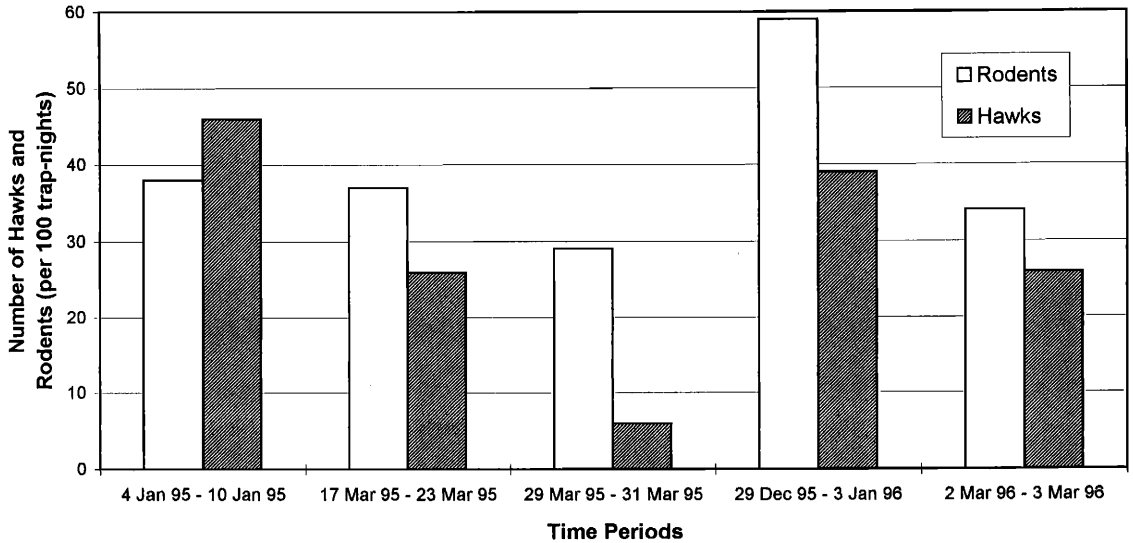
Figure 2. Total number of Red-tailed Hawks recorded during raptor surveys compared to rodent abundance indices in rice fields and roadsides sampled within the same time periods.
