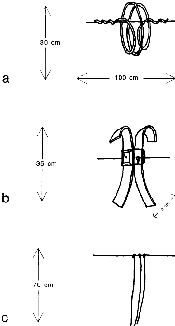
FIGURE 2. The three different wire markers studied: a. White spiral on static wire (30 cm \times 100 cm), b. Black crossed bands on conductors (35 cm \times 5 cm), and c. Black stripes on conductors (70 cm \times 0.8 cm).
