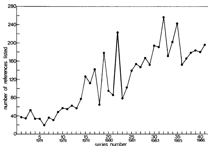
Figure 1. Increase in the number of references listed in "Recent Publications on Waders" since its inception.
