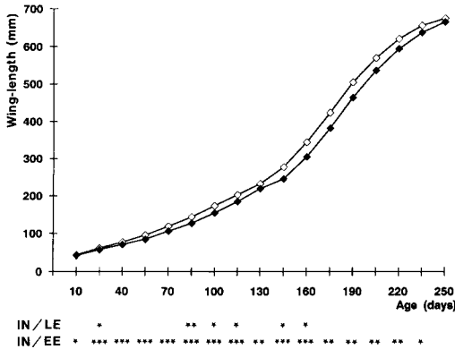
FIGURE 3. Changes with age in wing length of Wandering Albatross chicks fledged by inexperienced parents (IN: black squares) and parents with an extensive experience (EE: white squares). Values obtained for the chicks of parents with a limited experience (LE) are virtually identical to those of the chicks of EE parents. Significant differences between chicks of IN, LE, and EE parents are indicated by asterisks at 15-day intervals (Student's t -test: * = P < 0.05 , ** = P < 0.01 , *** = P < 0.001 ).
