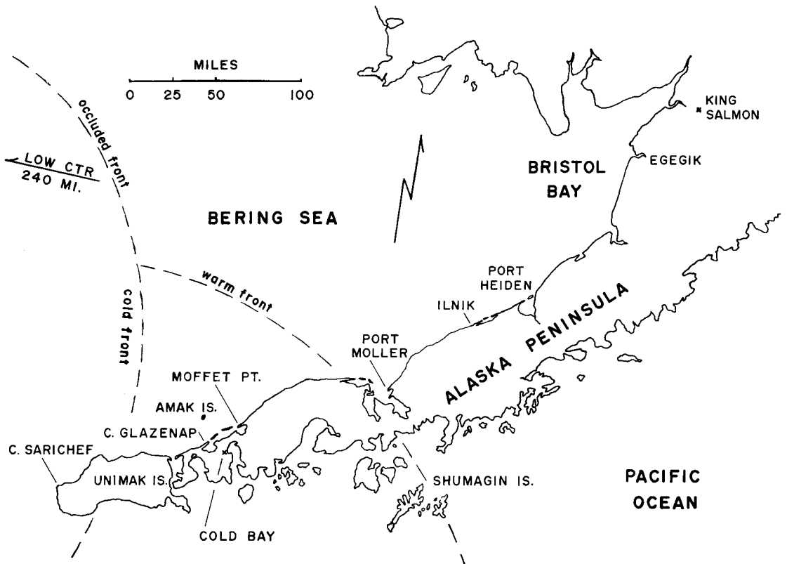
FIGURE 1. Alaska Peninsula and Unimak Island with surface weather on 22 April 1970.
