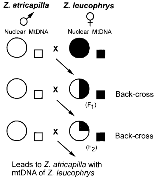
FIG. 4. Diagram of a hypothetical hybridization process showing how back-crossing to the paternal donor could ultimately yield a population with Z. leucophrys mtDNA and a Z. atricapilla nuclear genome. Nuclear genomes are represented by circles and mtDNA genomes are represented by squares. Zonotrichia leucophrys DNA is represented by blackening of the circle or square (e.g. a half blackened circle contains one half Z. leucophrys and one half Z. atricapilla nuclear DNA).
