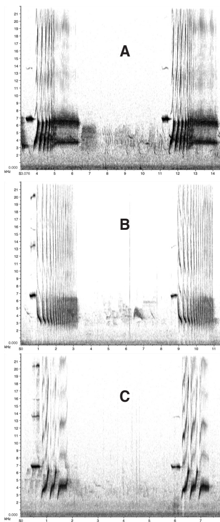
Figure 4. Some songs sung by the hybrid Brewer's × Black-chinned Sparrow in Cuyamaca Rancho State Park, California, 9 June 2007. A, Most frequent song, in which the pattern of the Black-chinned's song seems overlaid over the quality of a Brewer's song. Note the layers of harmonics in the terminal trill, as in Brewer's but not as in the Black-chinned. B, Song resembling a typical Black-chinned Sparrow's song, with the terminal trill shortened. C, Song consisting of three trilled notes in the cadence of the first three notes of a typical Black-chinned Sparrow's song. Again, note the harmonics. To hear 2 minutes, 50 seconds of the bird singing various variations, go to www.sdnhm.org/research/birds/hybrid.html .
